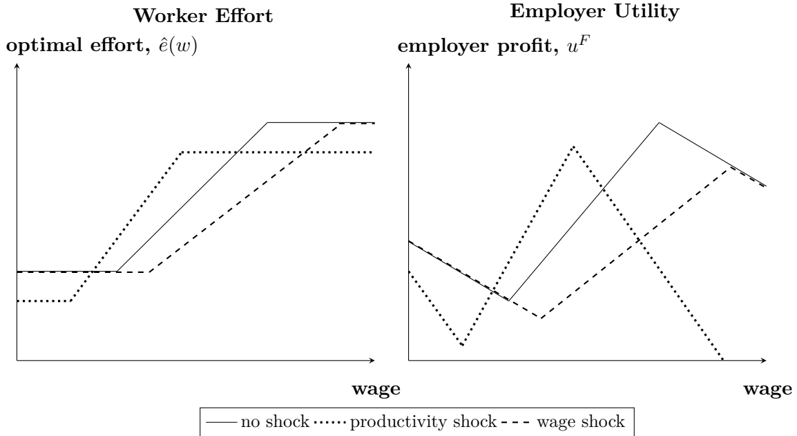
Figure 3: The Effects of Shocks
